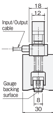
FGMH-4A (Single axis)
