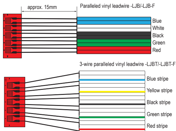
FYV 5-element single axis integrated
