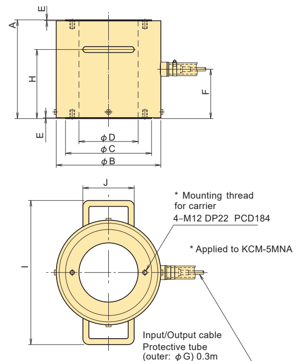
KCM-2MNA~ 5MNA
