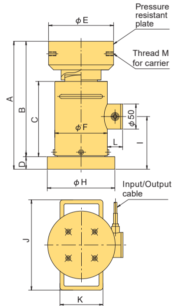
CLJ-5MNB, -10MNB
