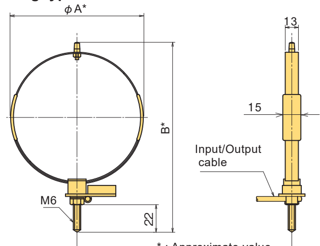
Ring type
