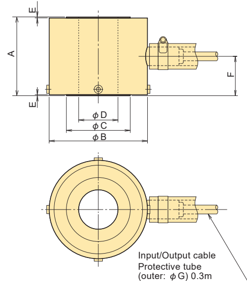
KCM-2MNA~ 5MNA
