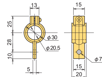
HOLDER CDPF-11-25
