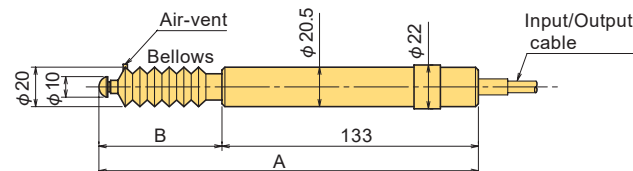
HOLDER CDPF-11-25
