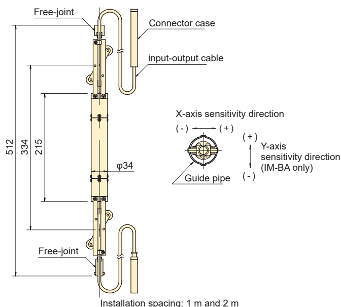
IM-10UA (1-axis) / IM-10BA (2-axis)
