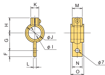
HOLDER CDPF-11
