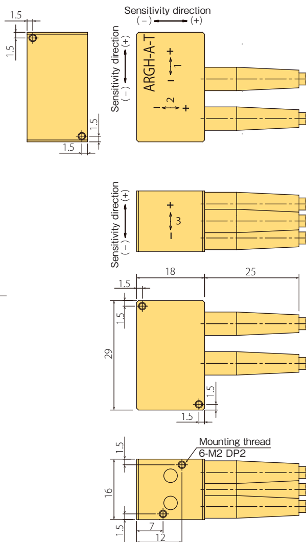
Acceleration transducer
